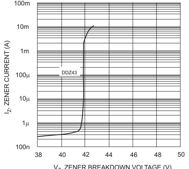
Fig. 9 Typical Reverse Characteristics, DDZ43
